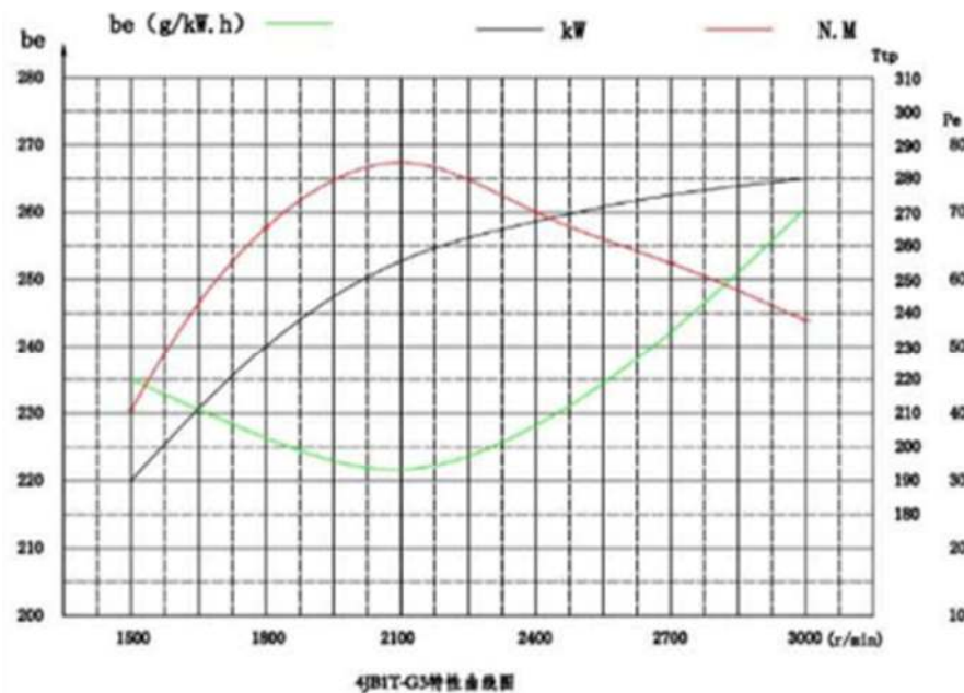
4JB1T-G3 CURVE
