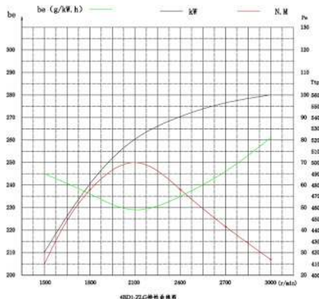
4BDZL CURVE
